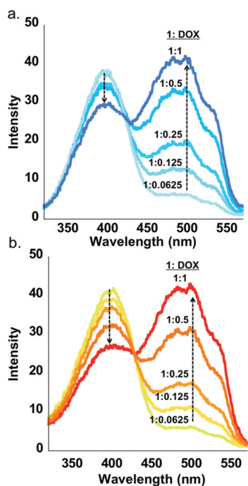
Fig. 3 Overlaid excitation spectra (590 nm) of 1_{12}15 (5 mM mixture in a LiPB pH 7.4) with increasing amounts of the acceptor DOX showing the quenching of the former (donor) with the concomitant increase in intensity for the latter (acceptor) as indicated by the trend arrows; (a) sample without and (b) with 1 M KCl.
