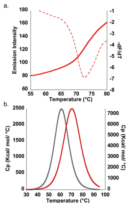
Fig. 4 Melting profiles for \text{hSGQ}\cdot\text{DOX} (LiPB pH 7.4) as determined by (a) variable temperature FRET experiments, monitoring the donor emission at increasing temperatures. The reported T_m is the inflection point in the melting profile as determined by the minimum in the first derivative plot (dashed red line). (b) Overlay of the DSC endotherm for \text{hSGQ} (grey curve) and for \text{hSGQ}\cdot\text{DOX} (red curve), showing an enhancement in the thermal stability of the hexadecamer when interacting with the drug.
